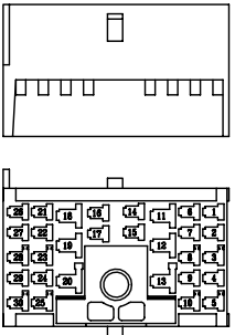
CONNECTOR SHOWN AT ACTUAL SIZE FOR LABELLING CLARITY
